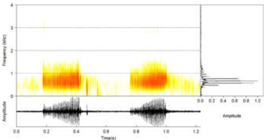
Figure 3. (a) oscillogram, and (b) audiospectrogram of a single note of the advertisement call of Odontophrynus cultripes from São Tomé das Letras, state of Minas Gerais, Brazil.
