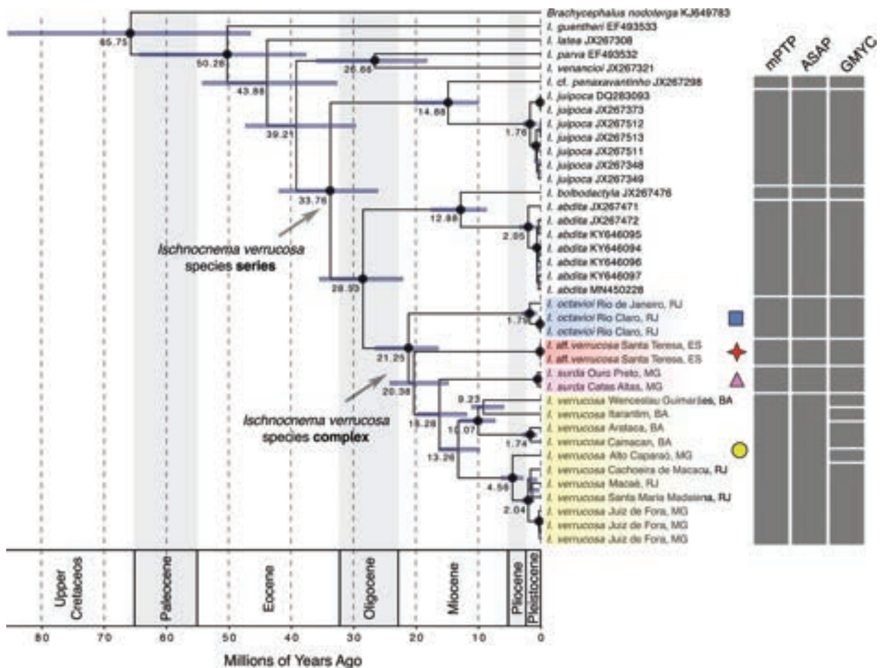
Figure 2. Bayesian chronogram for the Ischnocnema verrucosa series based on analysis of the mitochondrial 16S gene. Circles on nodes denote significant posterior probability ( pp = 0.95\text{--}1.0 ). Median ages in millions of years are shown on nodes, and 95% HPDs of node ages are indicated by horizontal blue bars. Vertical gray bars on the right represent the species delimited by GMYC (Generalized Mixed Yule Coalescent), mPTP (multi-rate Poisson Tree Processes), and Assemble Species by Automatic Partitioning (ASAP).
