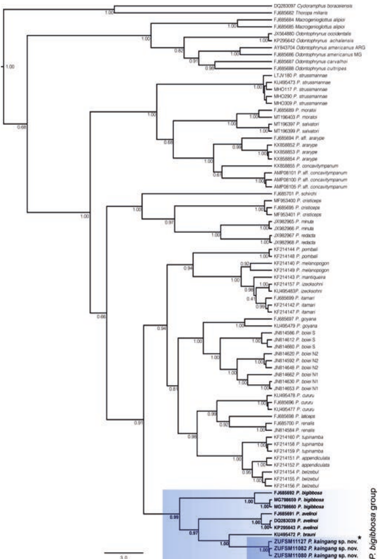
Figure 6. Gene tree based on phylogenetic analysis of the 16S mtDNA gene for the 28 species of the genus Proceratophrys . Scale indicates rate of base substitutions per site.
