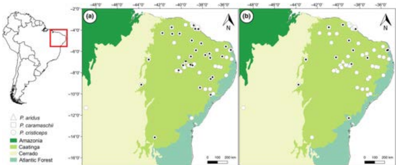
FIGURE 1 (a) Sample localities for morphological (circles, triangles and squares) and molecular (dotted) data. (b) Sample localities for morphological (circles, triangles and squares) and acoustic (dotted) data. Detailed locality information is shown in Table S2
